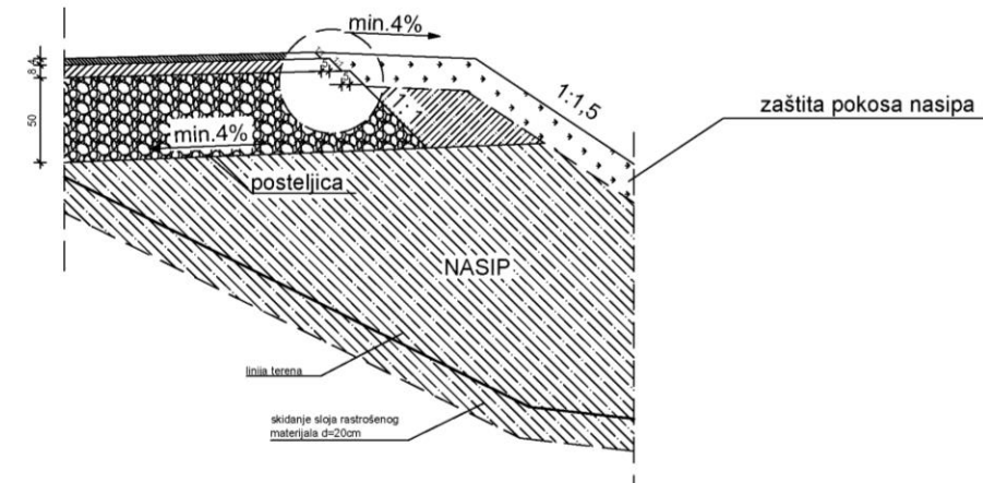
DETALJ BANKINE MJ 1:25
